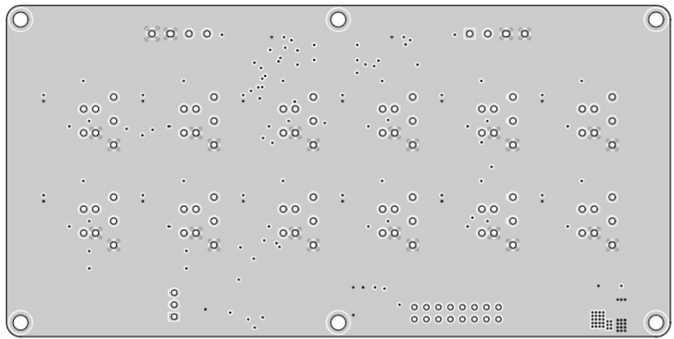
Power Plane
