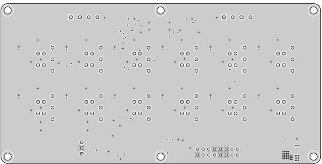
Ground Plane
